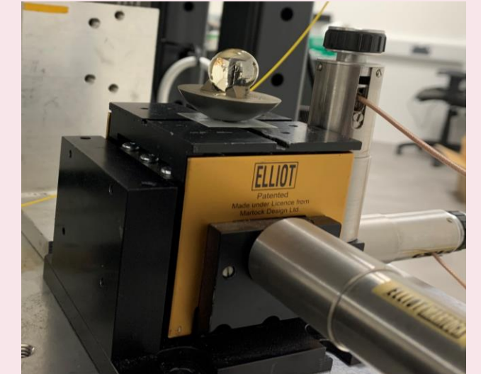
Signal generated by the signal generator stimulate the target movement by changing the OPD of the retro reflector using Elliot piezo vibrator.
